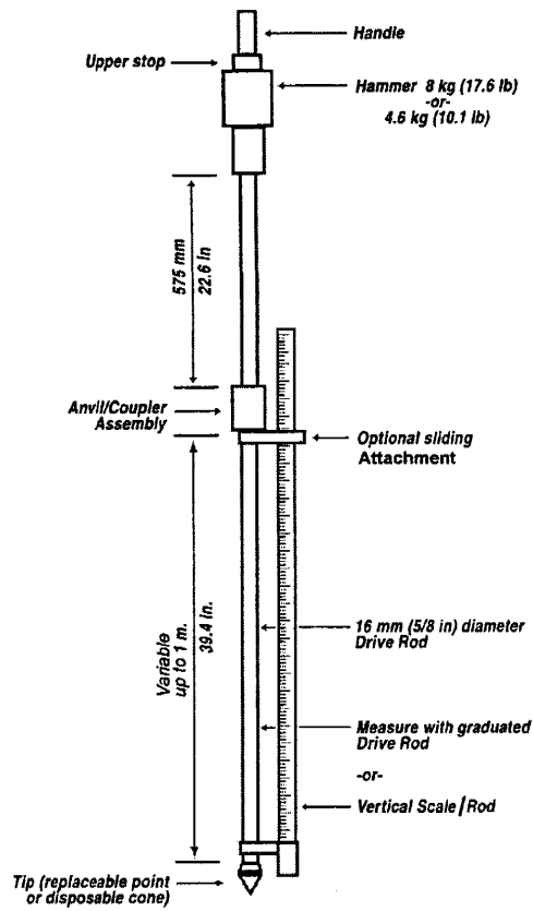
Figure 1 - Schematic of DCP Device
